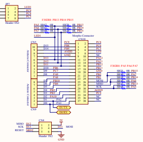
Extension connectors
