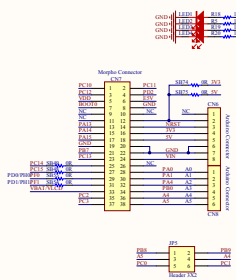
Extension connectors
