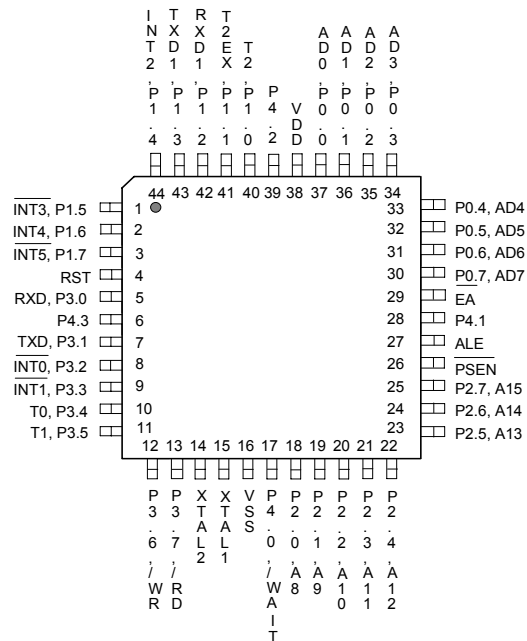
44-Pin QFP
