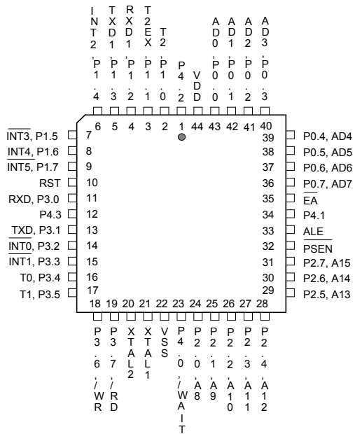
44-Pin PLCC
