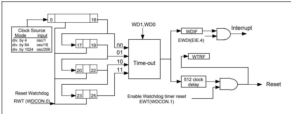
Figure 19. Watchdog Timer
