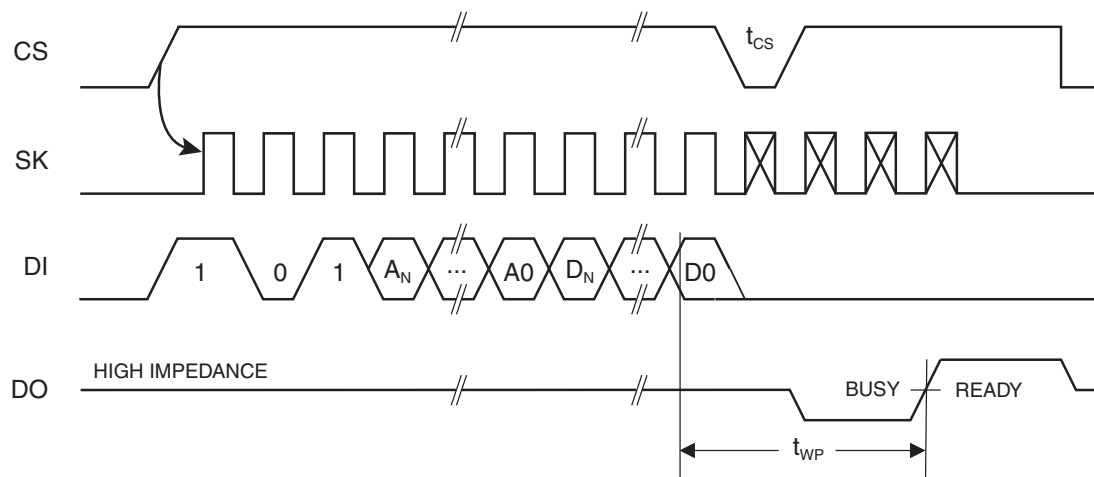
Figure 5-5. WRITE Timing
